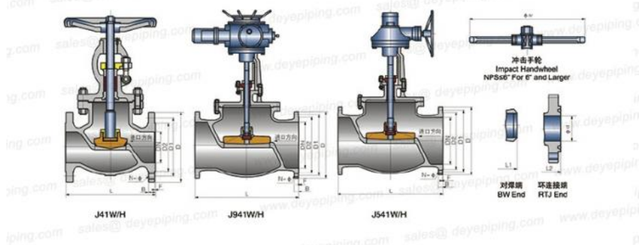
美标150Lb铸钢截止阀 Class 150 Cast Steel Globe Valve
